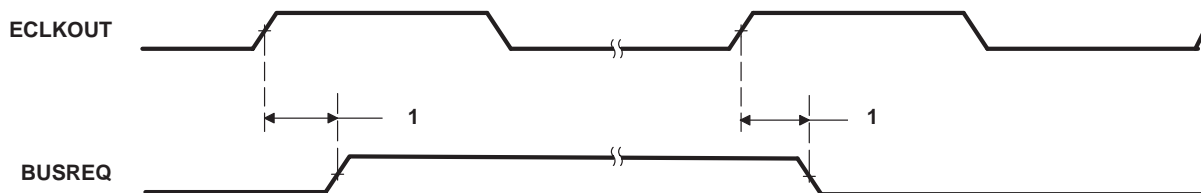
Figure 38. BUSREQ Timing
